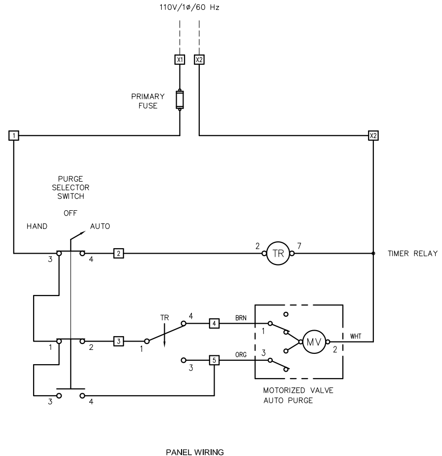
PANEL WIRING
